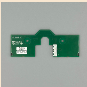
Tray Sensor PCB
