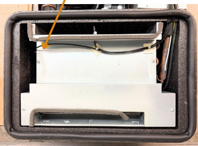
EVAPORATOR PROBE
